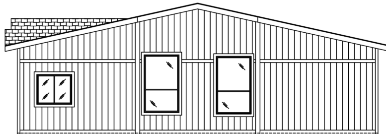
FRONT ENDWALL
